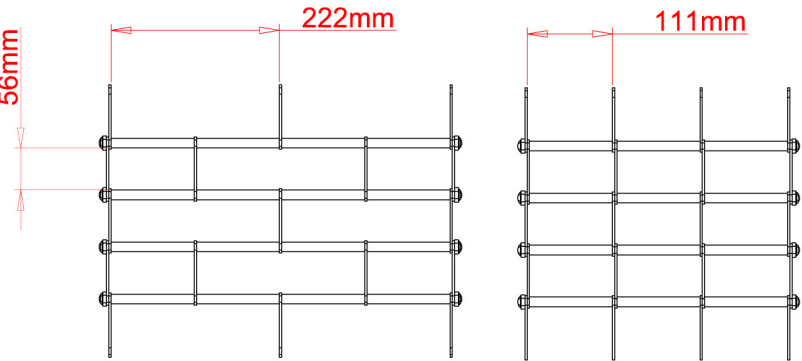
Brick-bond arrangement
