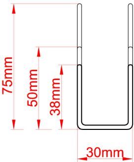
38 / 50 / 75mm Aluminium U-Channel guide (affixed to box section or angle)
